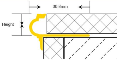
Aluminium Stair Nosings
