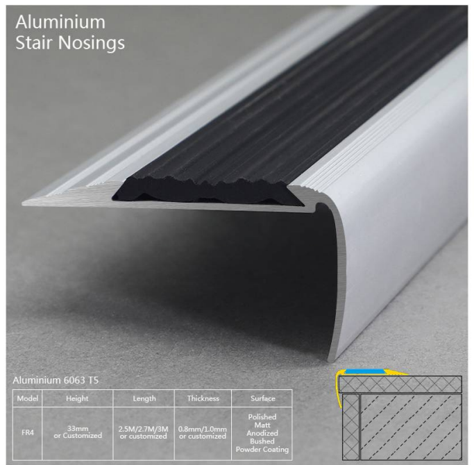
Aluminium Stair Nosings
